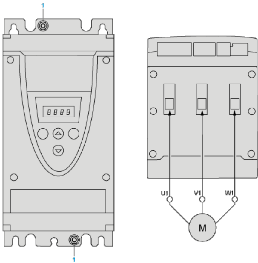
1 Ground connection
