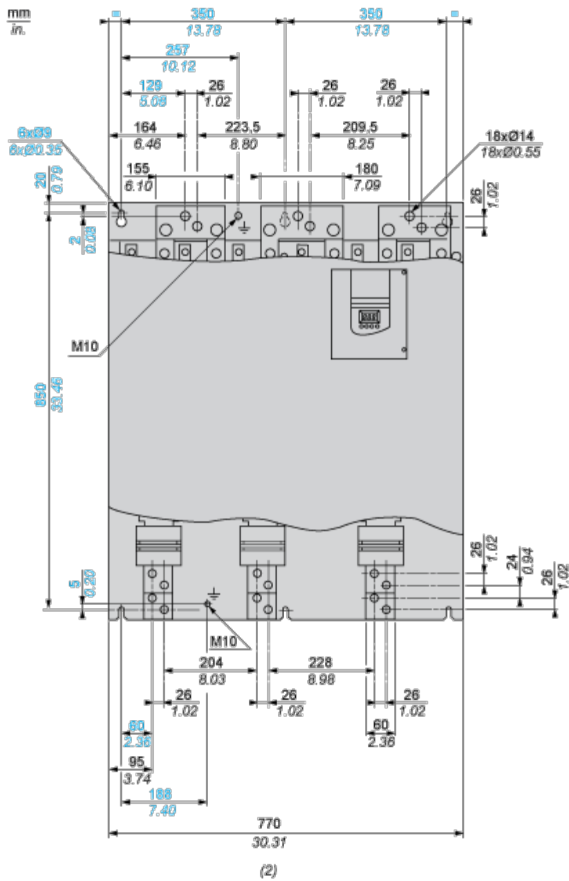
(1) Right View (2) Front View
