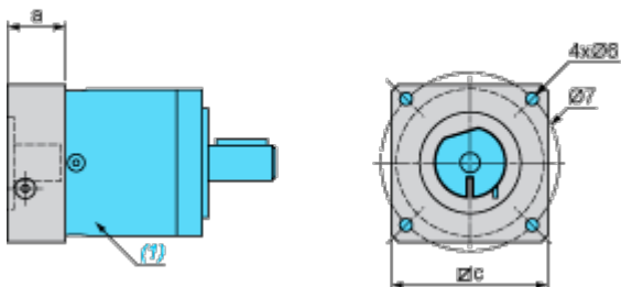
(1) Gearbox
