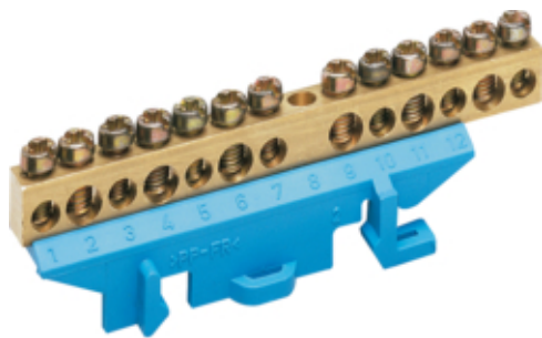
Brass terminal, 7x10mm 2 6x16mm 2 , N
